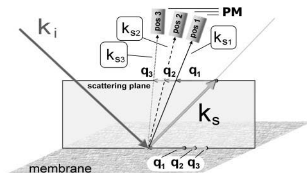
FIGURE 3 Schematic depiction of the scattering geometry used in our DLS setup, showing the incident vector k_i , the specular reflected vector k_s (reflection angle 45^\circ ), in-plane wave vectors q_1 < q_2 < q_3 , and the scattered vectors k_{s1} , k_{s2} , k_{s3} , which were detected by the photomultiplier (PM) at the corresponding angles ( pos1 , pos2 , pos3 ).
